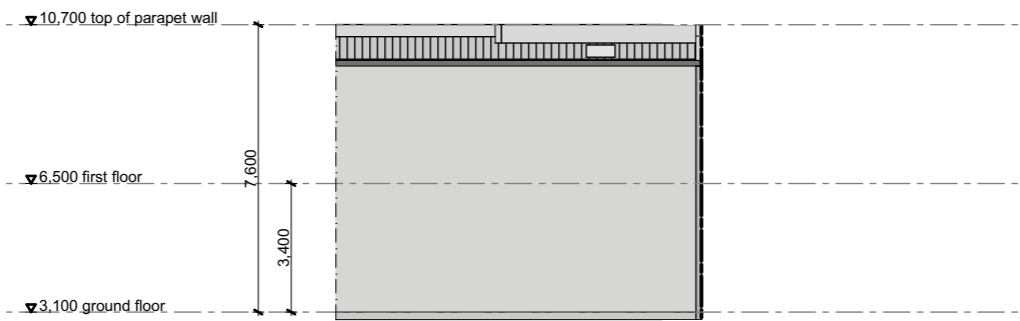
unit 243 elevation B
