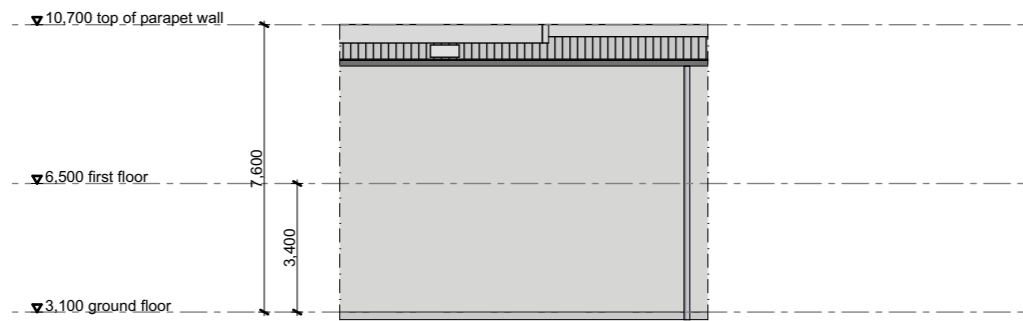
unit 242 elevation B
