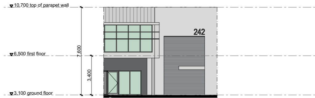
unit 242 elevation A
