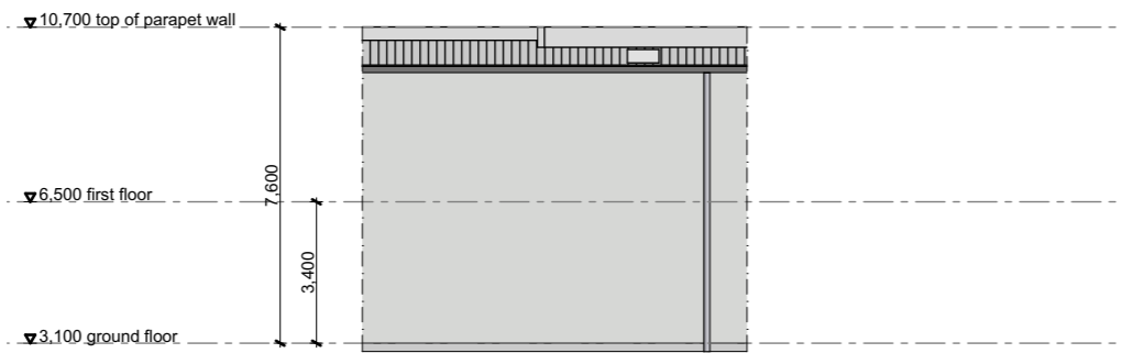
unit 241 elevation B
