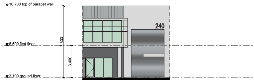
unit 240 elevation A
