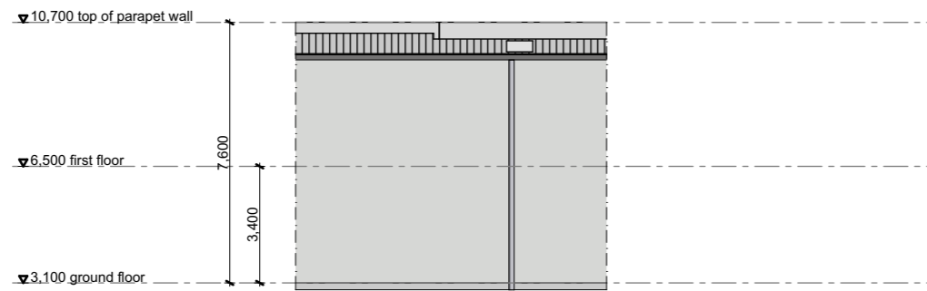
unit 239 elevation B
