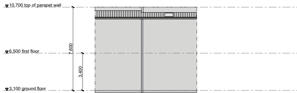
unit 237 elevation B
