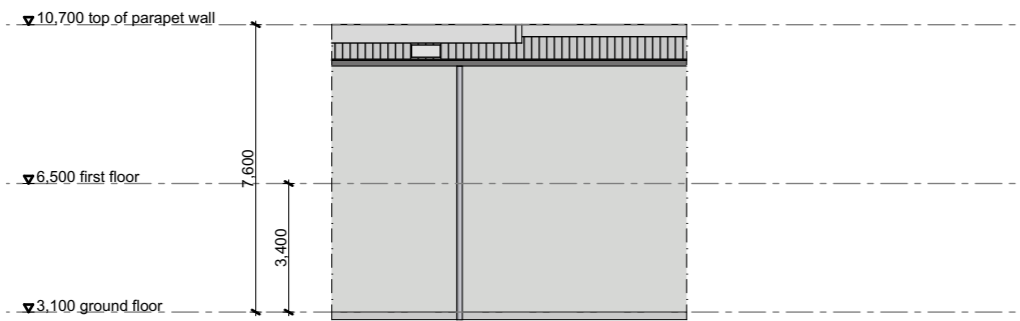
unit 236 elevation B
