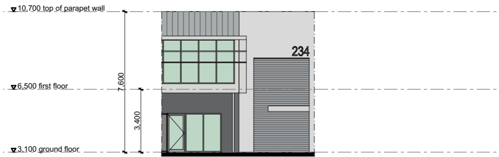
unit 234 elevation A
