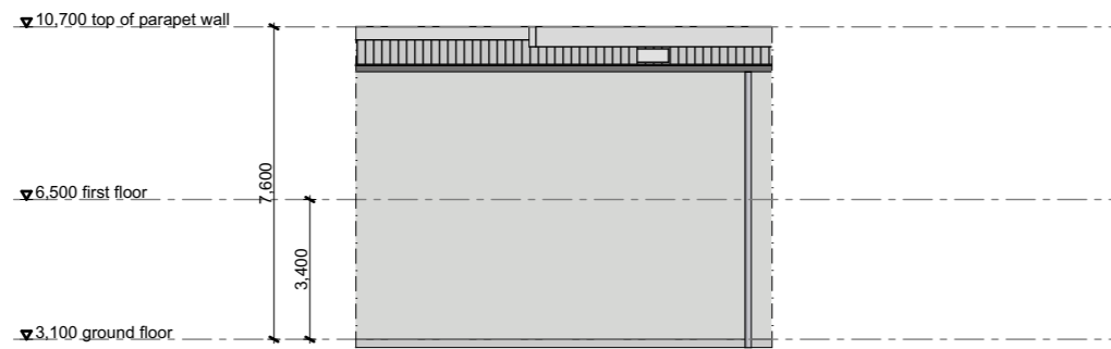
unit 233 elevation B
