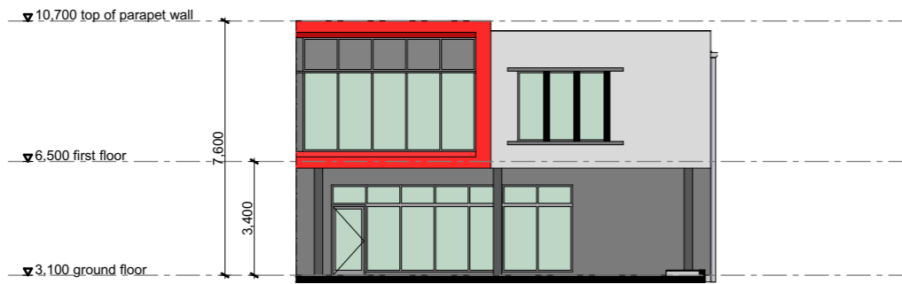
unit 231 elevation A
