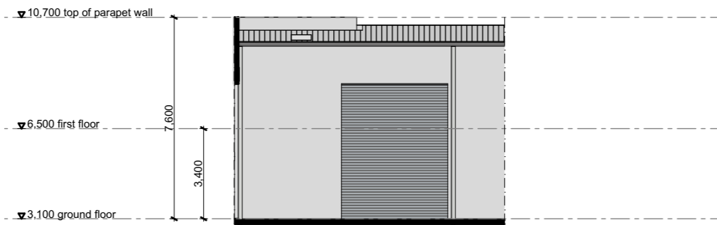
unit 230 elevation B
