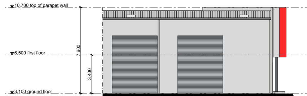
unit 229 elevation B
