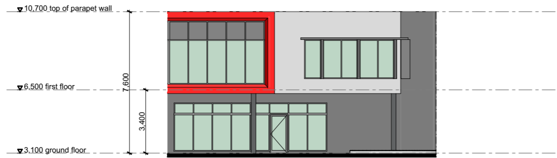
unit 228 elevation A
