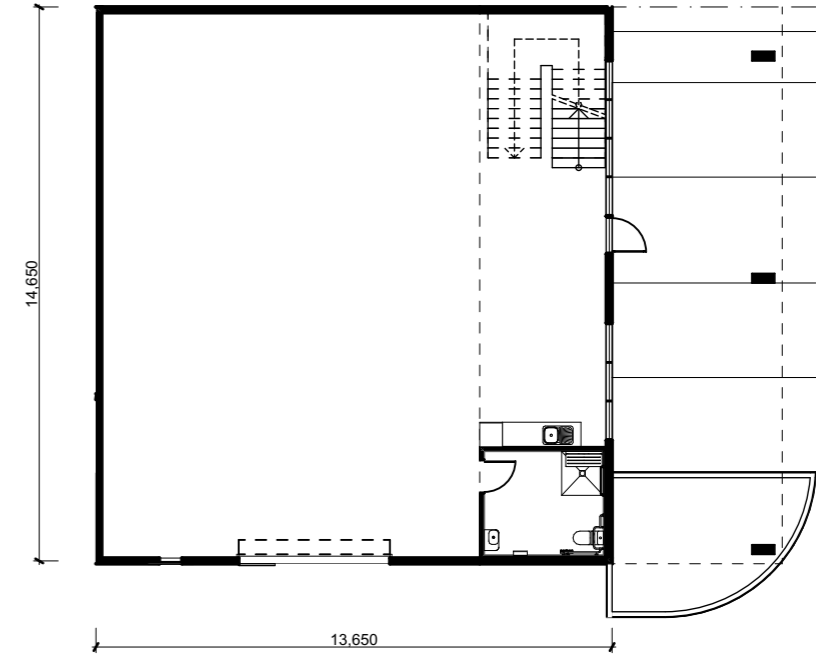
unit 227 ground floor plan
