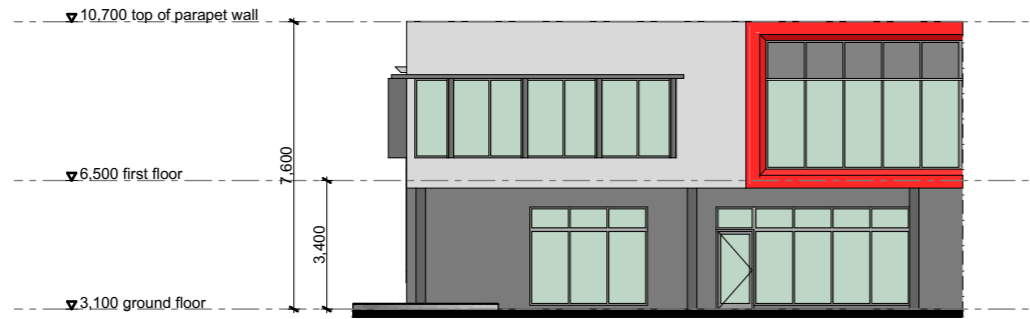
unit 227 elevation A
