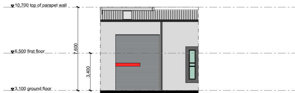
unit 226 elevation B
