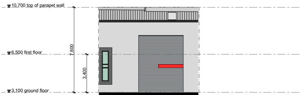
unit 225 elevation B
