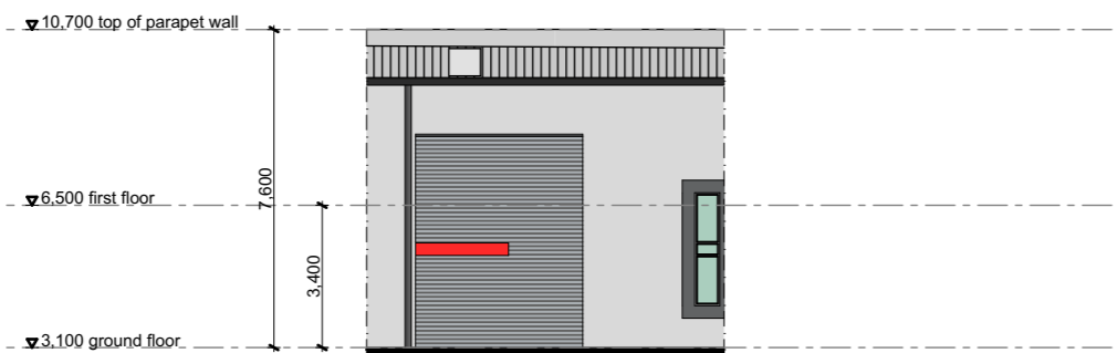
unit 224 elevation B
