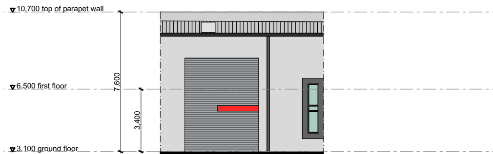
unit 222 elevation B
