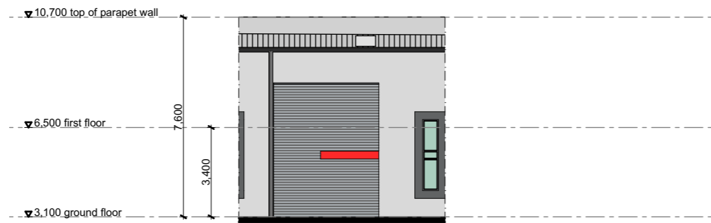
unit 219 elevation B
