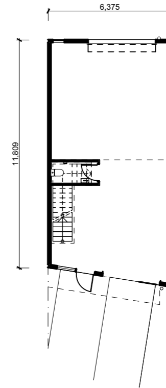
unit 217 ground floor plan
