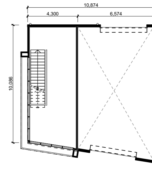
unit 216 first floor plan
