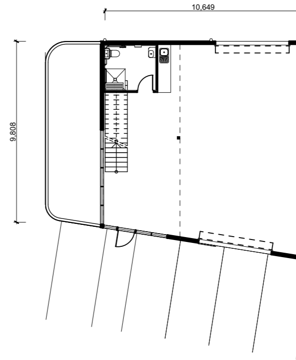
unit 216 ground floor plan
