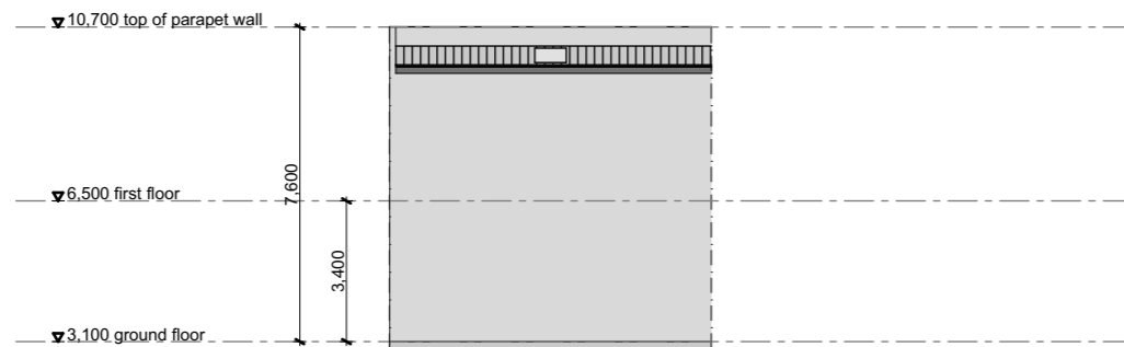
unit 214 elevation B
