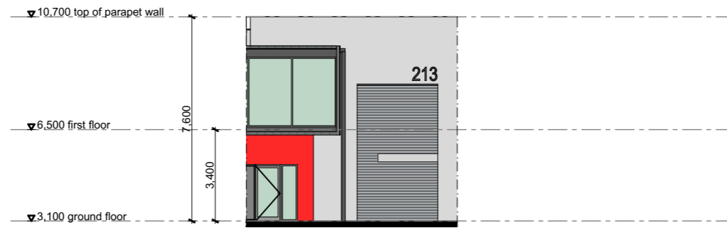
unit 213 elevation A
