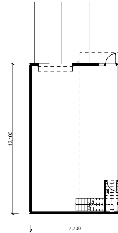
unit 213 ground floor plan
