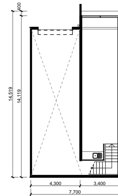
unit 213 first floor plan
