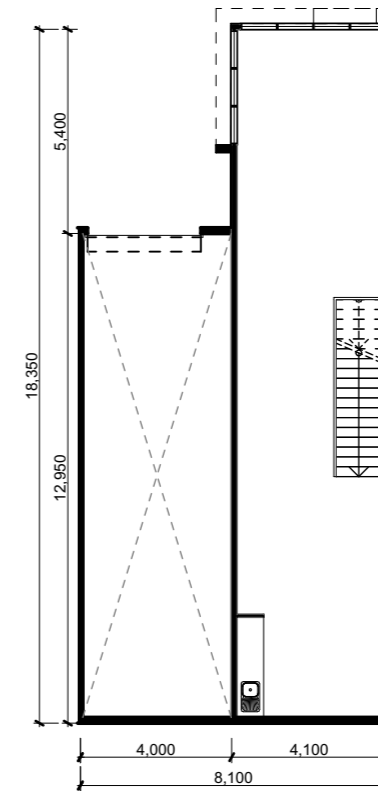
unit 211 first floor plan
