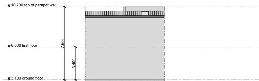
unit 210 elevation B
