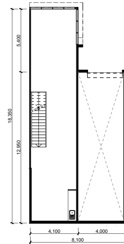
unit 210 first floor plan
