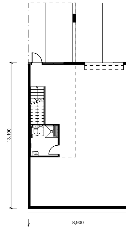
unit 208 ground floor plan
