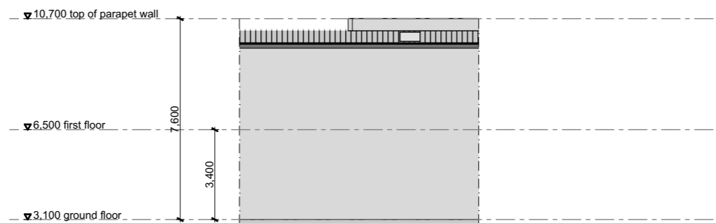
unit 208 elevation B
