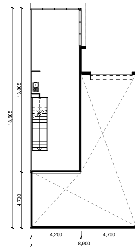
unit 208 first floor plan
