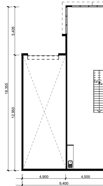
unit 207 first floor plan
