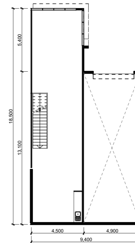
unit 206 first floor plan
