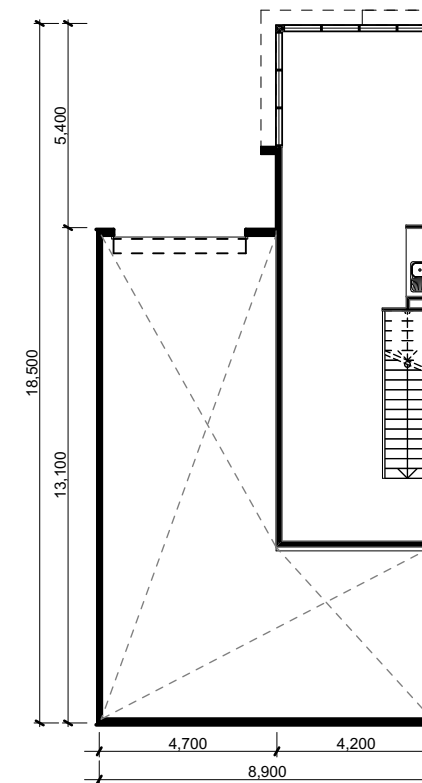
unit 205 first floor plan
