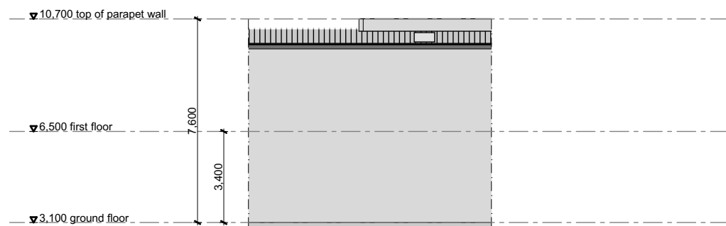
unit 204 elevation B
