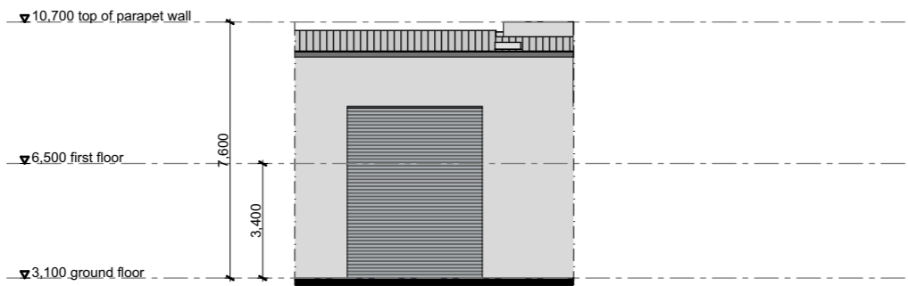
unit 202 elevation B
