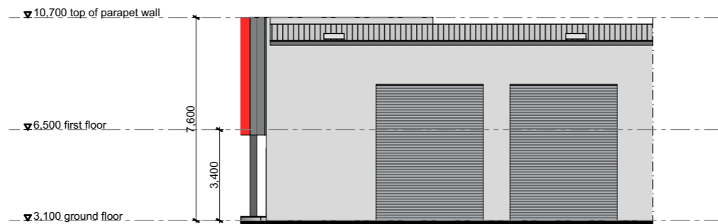
unit 201 elevation B
